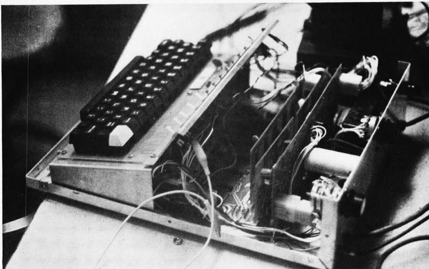
Southwest Tech CT-1024 video terminal . . . built on a homemade base. Row of switches along the top is for extra functions.
