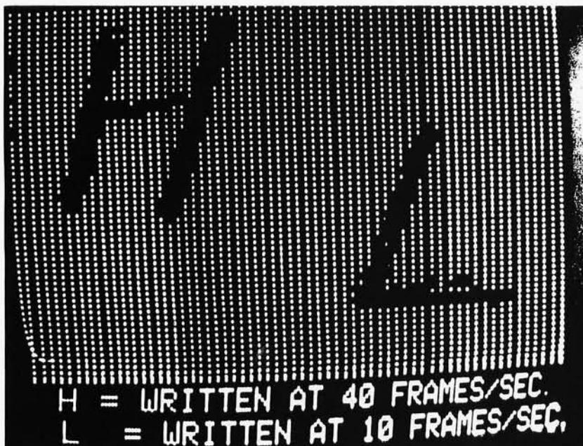
Photo 2: The light pen can be used in an "erase" mode by filling the screen with "on" dots then selectively removing dots with the light pen. The titles added to this picture (and all the pictures in this article) were created with a separate character generator which is not described.
